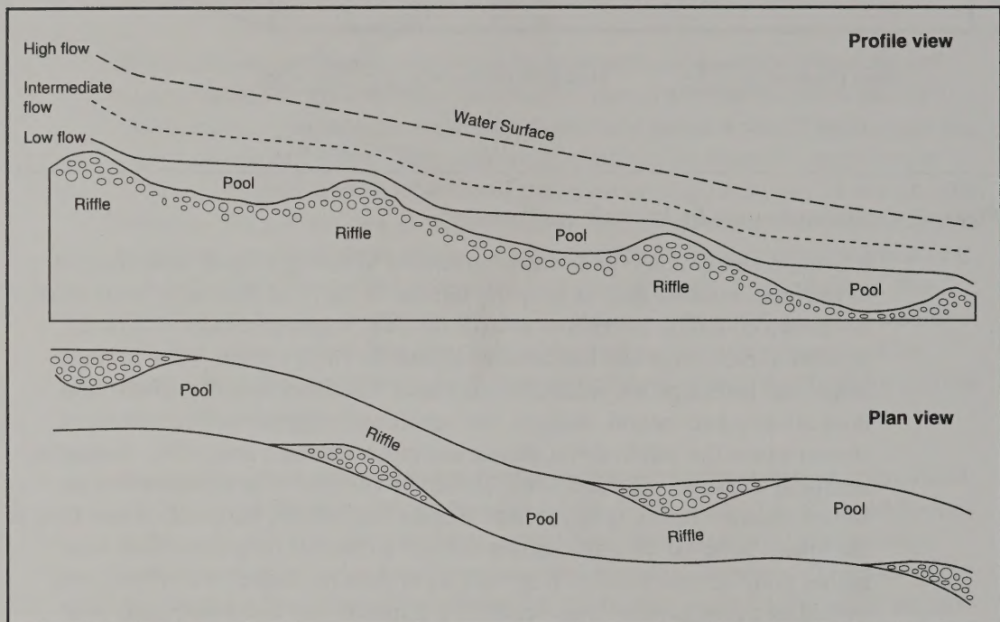
Figure 7. Diagram of longitudinal profile and plan view of a pool-riffle sequence. Water surface profiles in upper figure represent high, intermediate, and low flow conditions.
